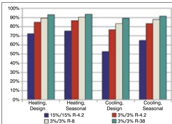
Figure 5 (left): Application of Standard 152 to an attic flex-duct system in Sacramento shows the attic duct efficiency. Figure 6 (right): Savings calculated with Standard 152 for changes to an attic flex-duct system in Sacramento.
